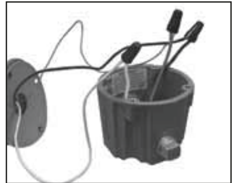
3. Attach fixture leads observing polarity; i.e.; braided bare copper wire-to-ground, white-to-common, and black-to-voltage.
